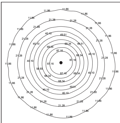
EWL-70 illumination on the floor expressed in lux in a room 5m x 5m with the lighting fixtures centrally placed at 3.5m in height
