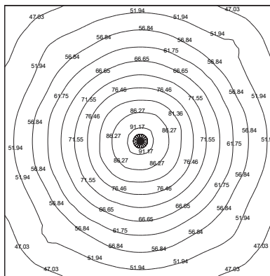
EWL-80 illumination on the floor expressed in lux in a room 5m x 5m with the lighting fixtures centrally placed at 5m in height
