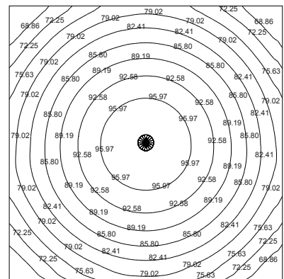
EWL-100 illumination on the floor expressed in lux in a room 5m x 5m with the lighting fixtures centrally placed at 7m in height.
