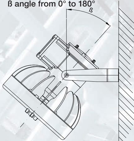
Example of wall mounting \beta angle from 0^\circ to 180^\circ
