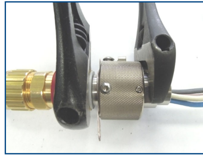
Tighten cable gland to rear shell as shown
